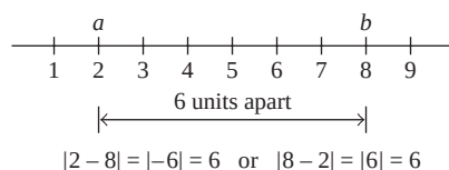
FIGURE 3 Distances in \mathbb{R} .
